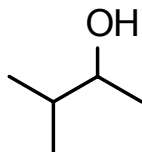
3-Methyl-2-butanol
