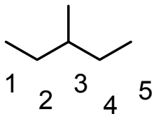
3-Methylpentan,
