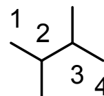
2,3-Dimethylbutan,
