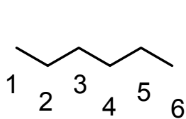
Hexan,
