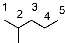
2-Methylpentan,
