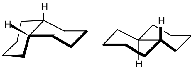
Isomere Bicyclo[4.4.0]decane
