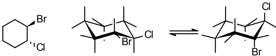
trans-1-Brom-2-chlorcyclohexan
