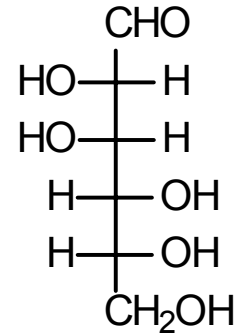
D(+)-Mannose,
