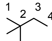
2,2-Dimethylbutan
