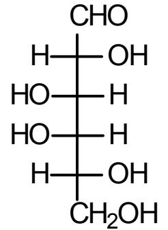
D(+)-Galactose
