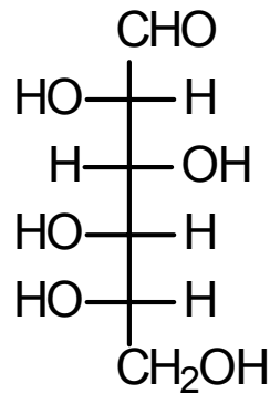
L(-)-Glucose
